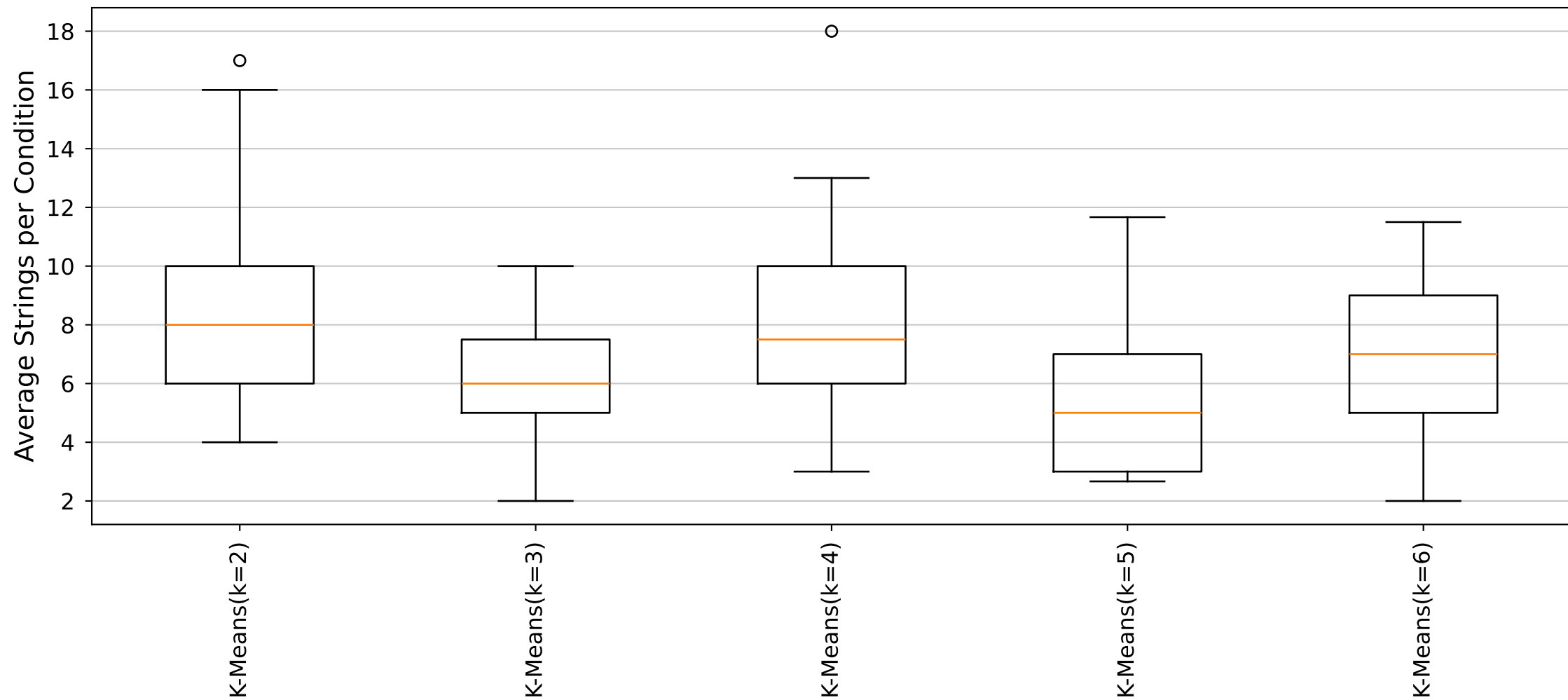
YARA Rules Average Strings per Condition Distribution (Cluster19_Size6 dataset)
